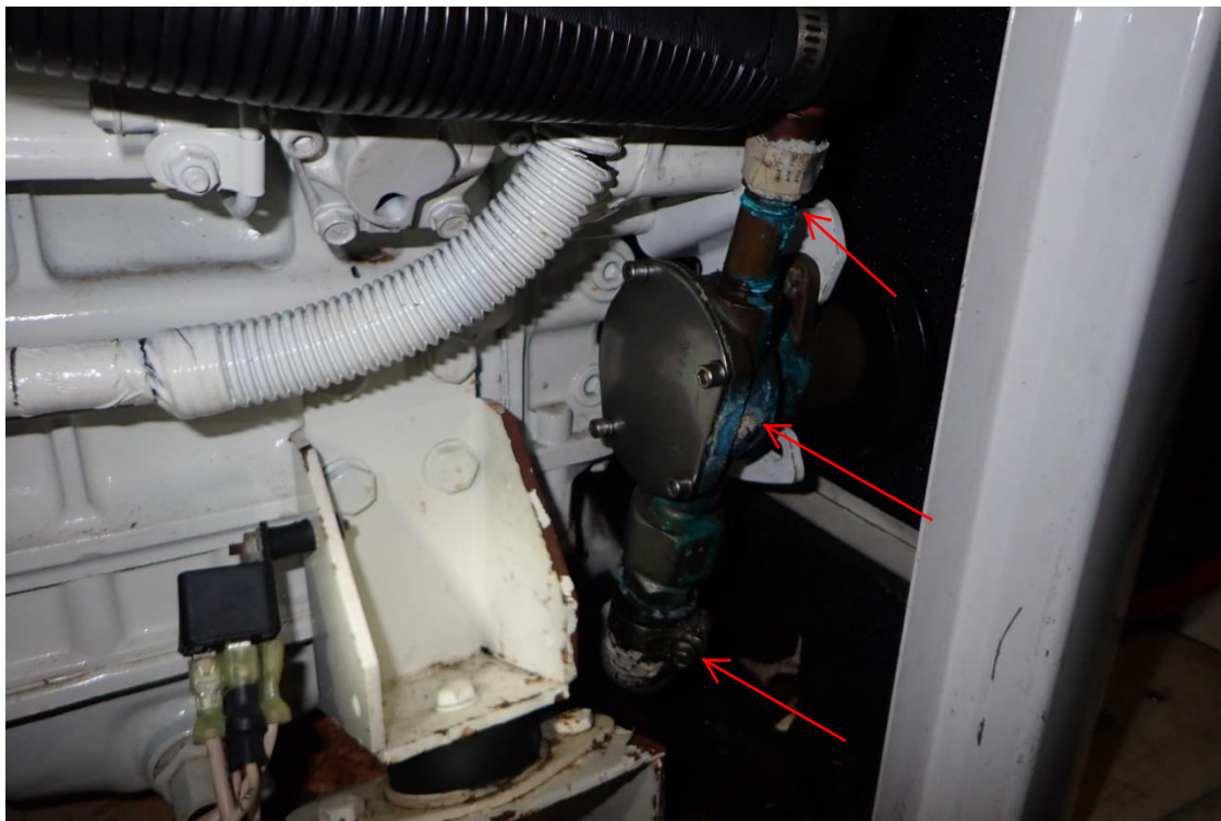
9. Leaking raw water pump at generator
