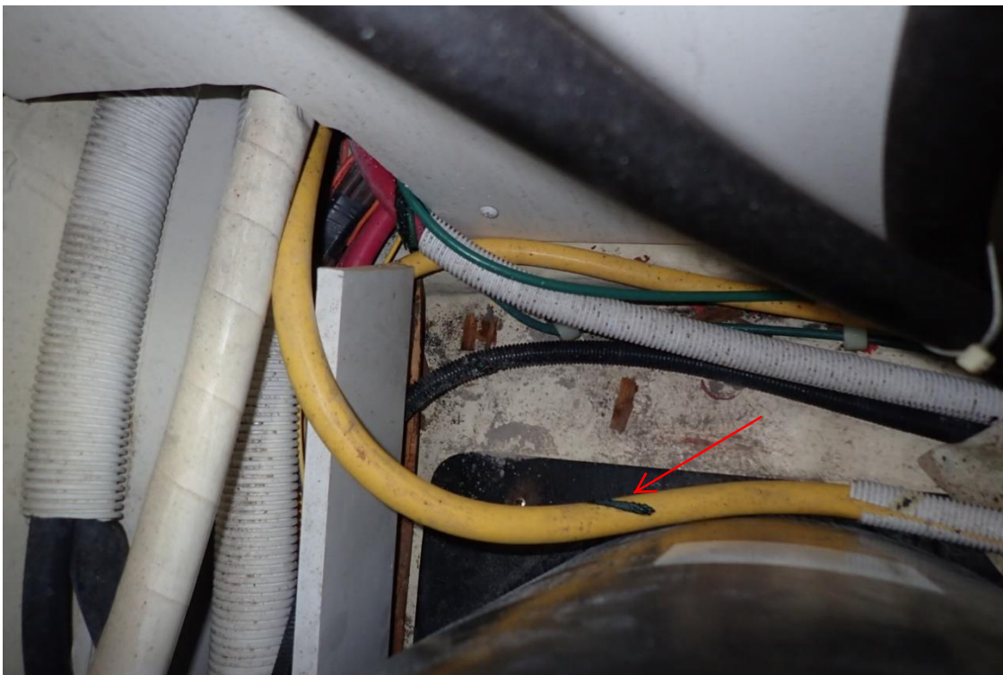
17. Overheating damage to battery cable, aft of starboard muffler
