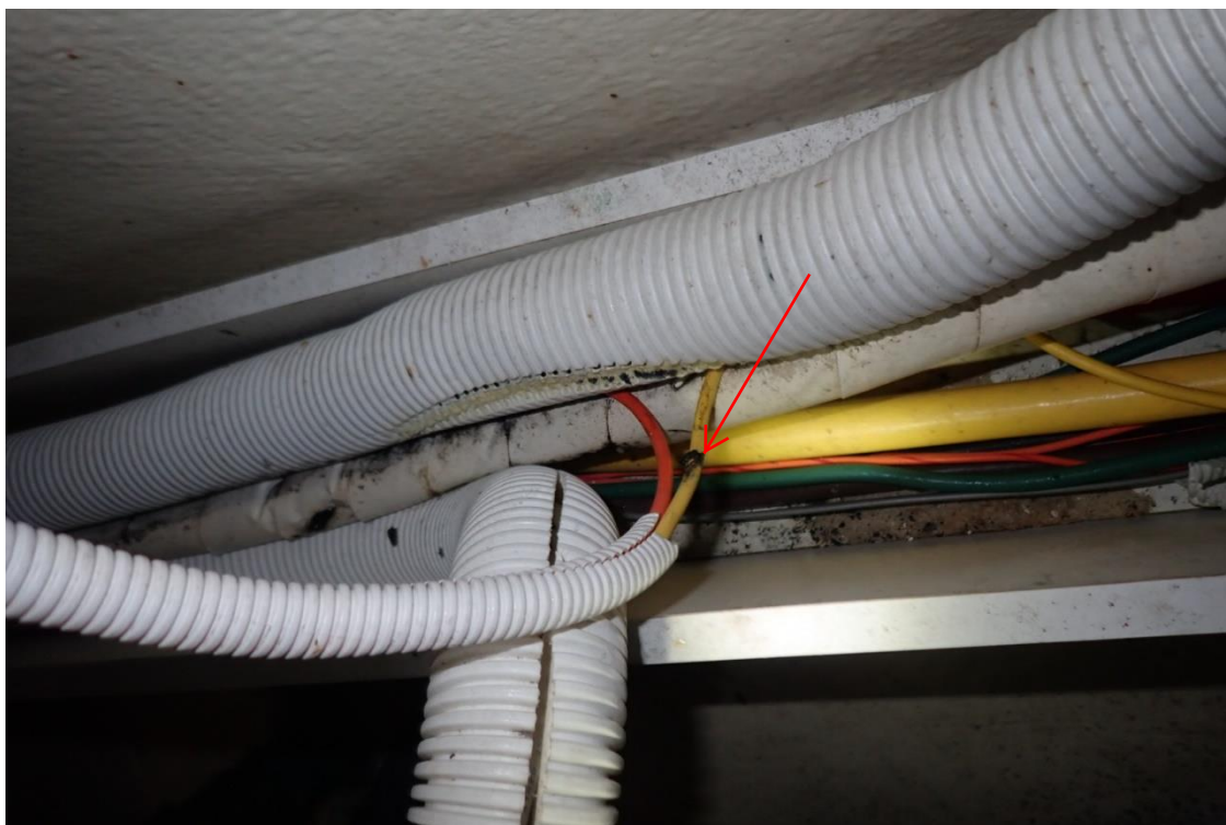
20. Overheating damage to wiring at starboard aft lazarette
