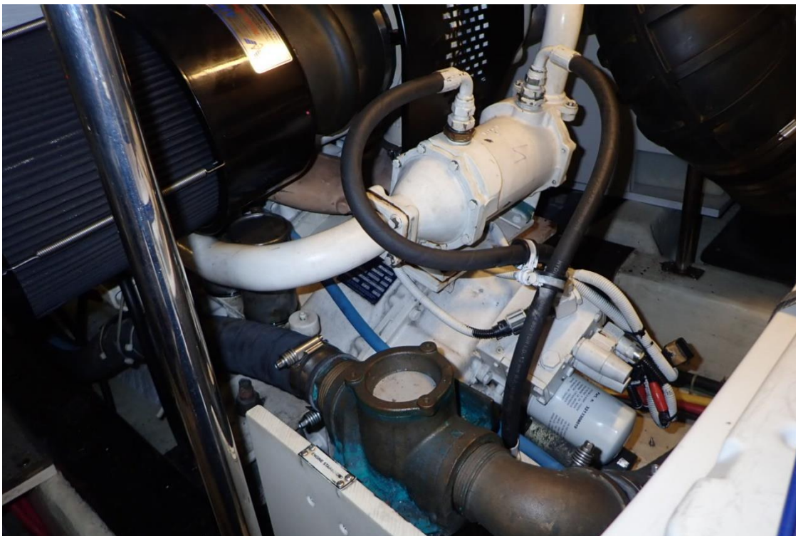
7. Starboard gear
