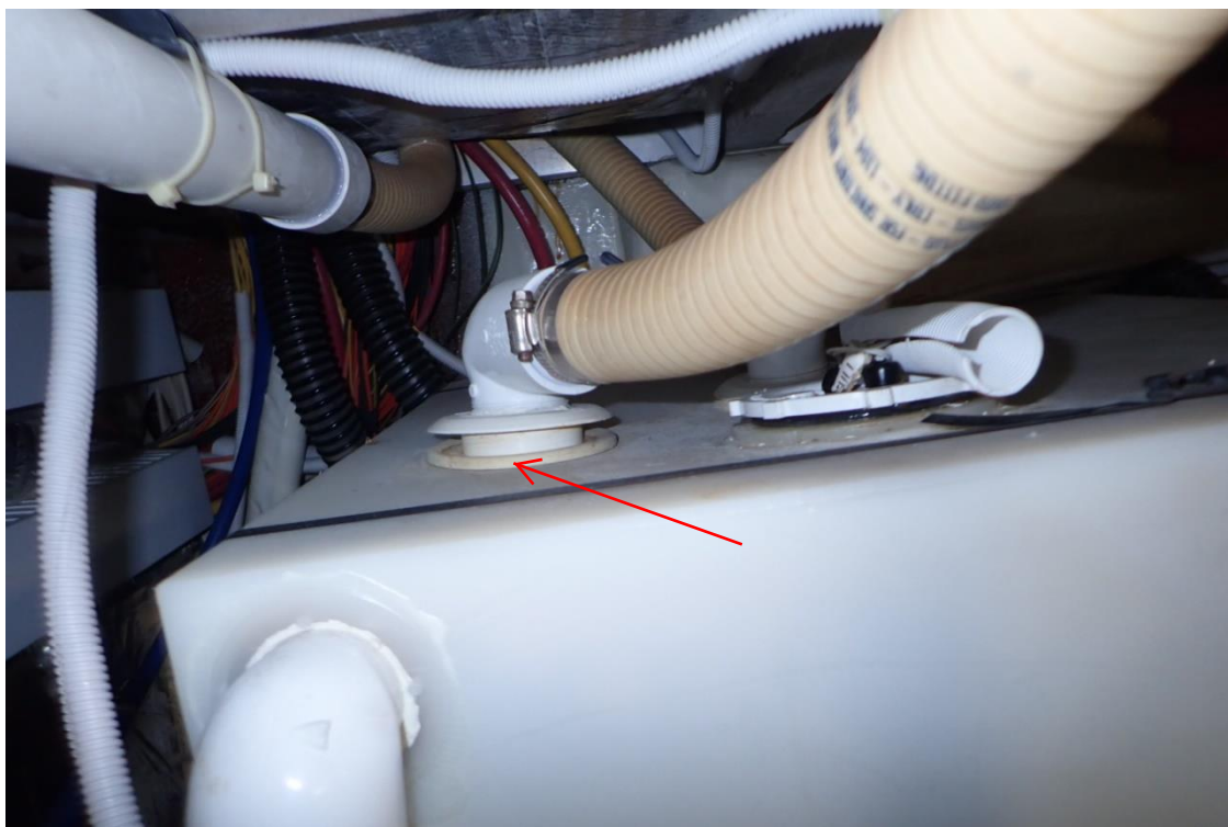
12. Loose fittings at starboard waste tank
