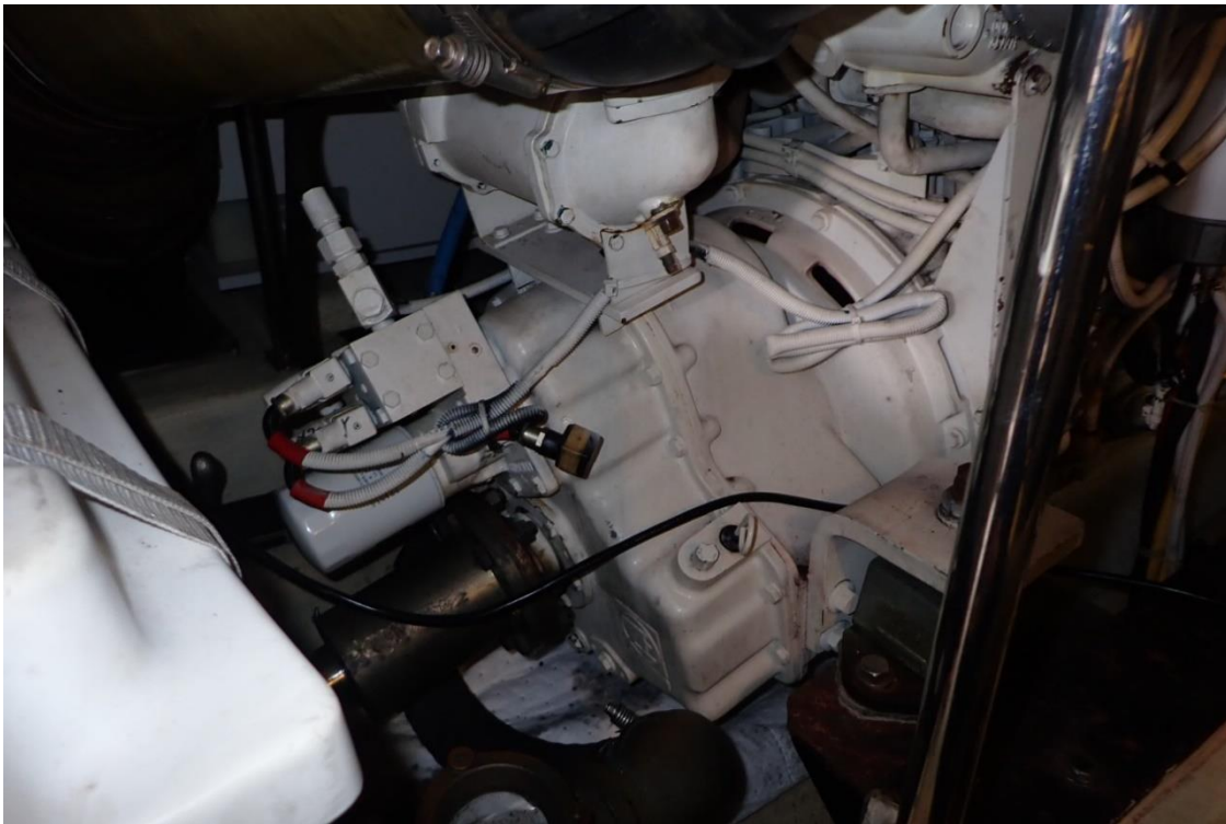
5. Port gear
