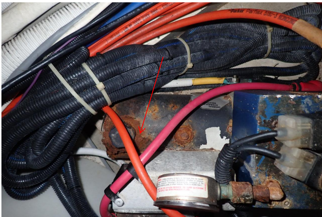
35. Corrosion at swim platform hydraulic pump
