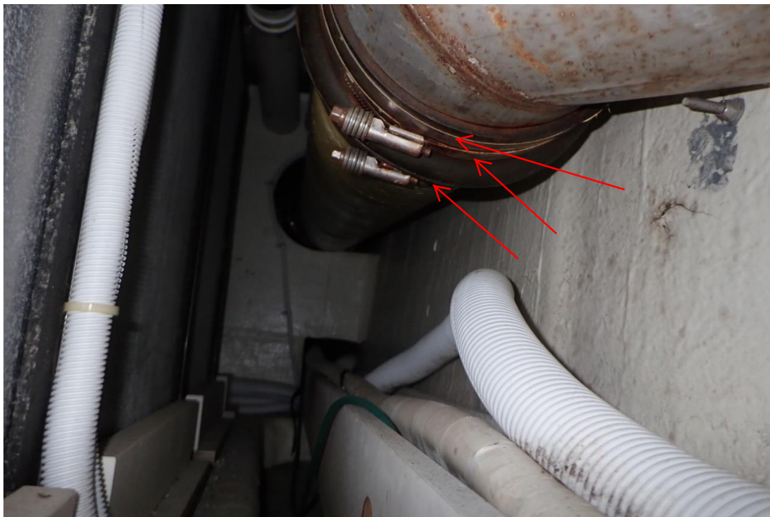
19. Corroding clamps at starboard exhaust thru-hull connections
