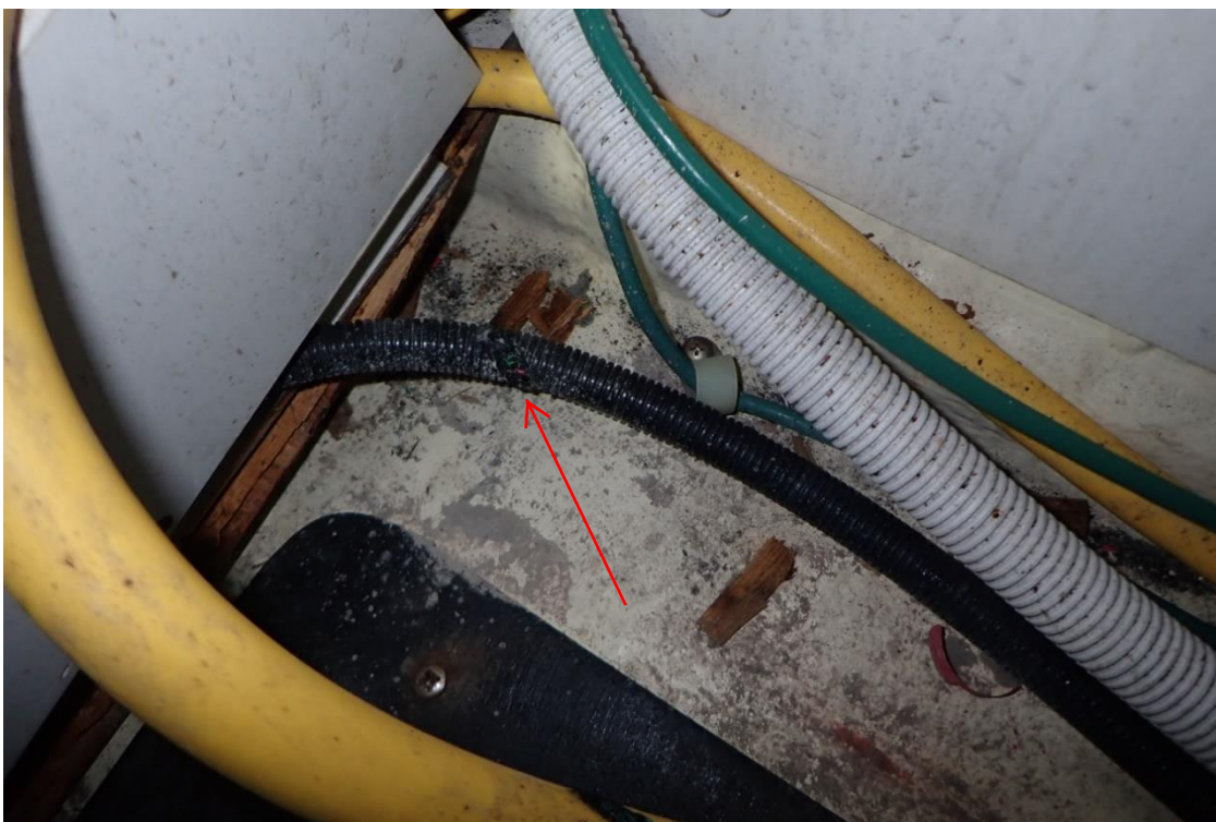
16. Overheating damage to wire loom, aft of starboard muffler
