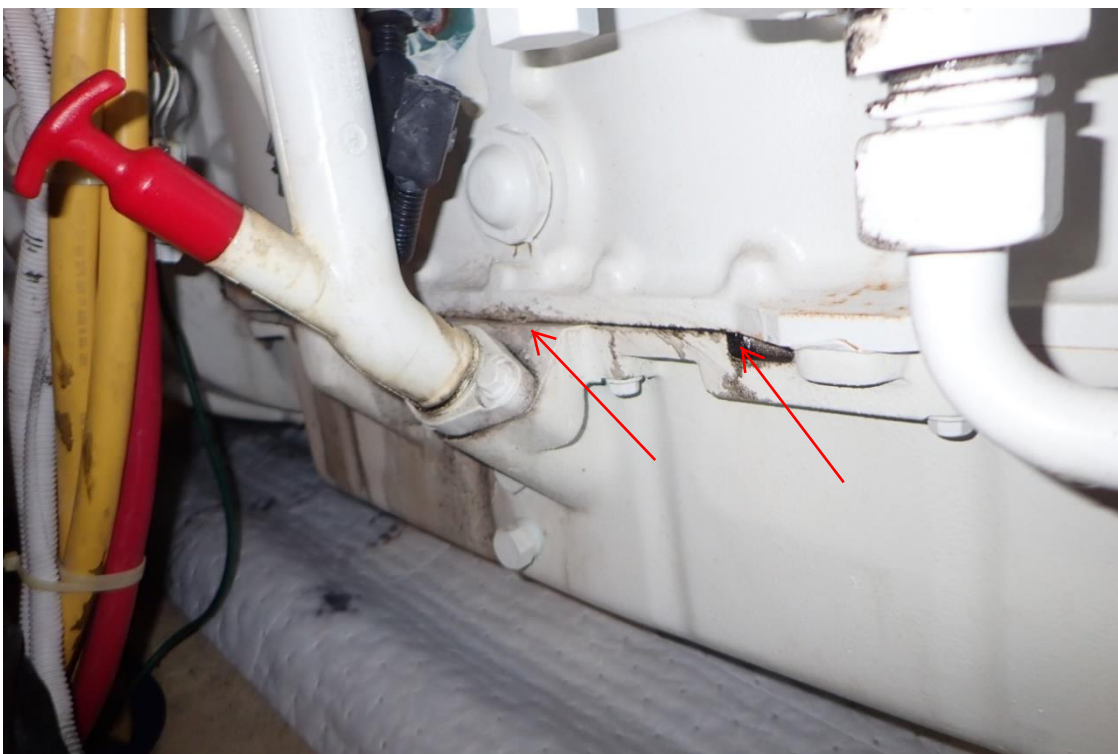
8. Oil leak at oil pan gasket, port engine
