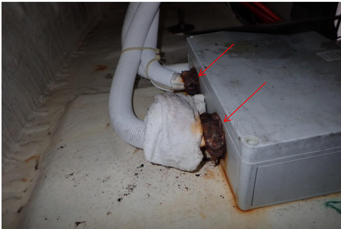
25. Corrosion at junction box in aft lazarette
