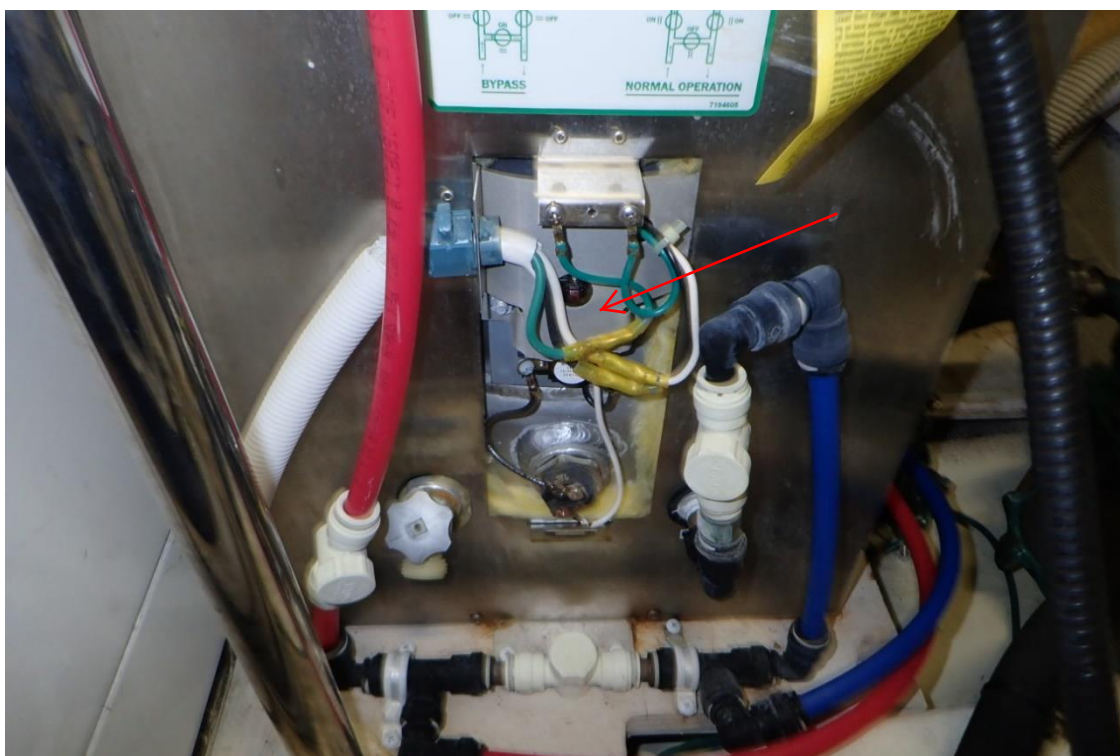
10. Cover removed from water heater panel
